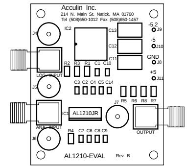
Component Layout
