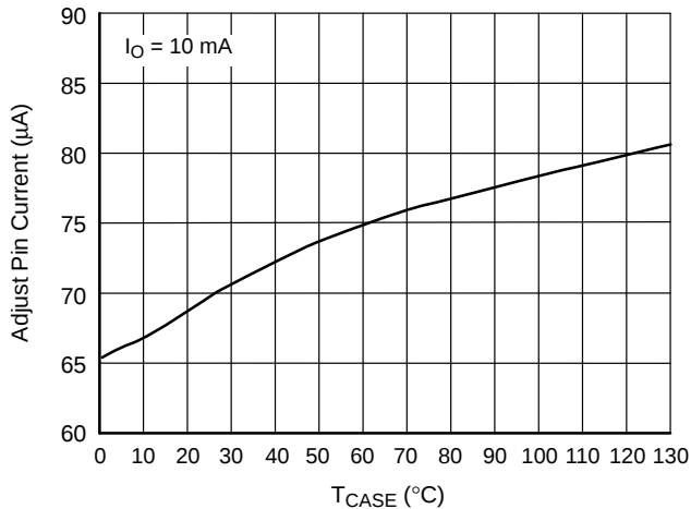
Figure 3. Adjust Pin Current Voltage vs. Temperature
