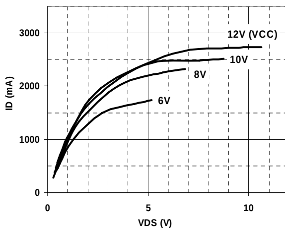
Figure 16. LDRV Pull-Down (Sinking)
