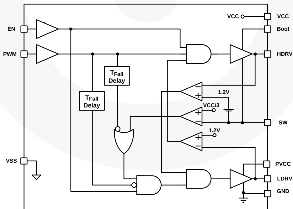
Figure 3. Functional Block Diagram, Each Side
