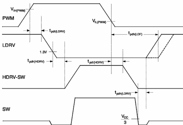
Figure 6. Adaptive Gate Drive Timing
