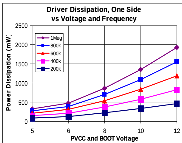
Figure 22. Driver Power Dissipation, One Side
