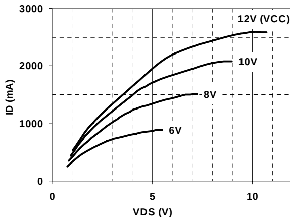
Figure 14. LDRV Pull-Up (Sourcing)
