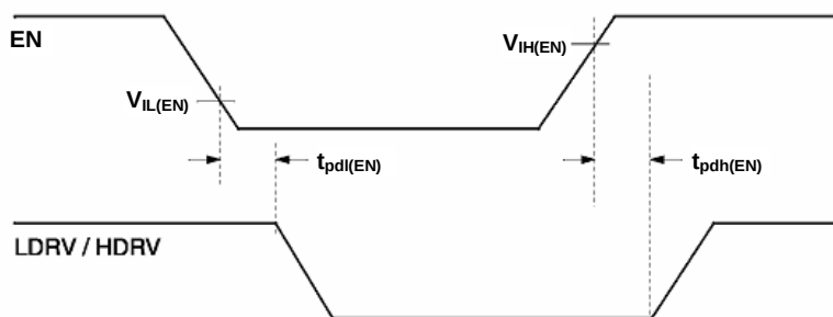
Figure 5. Enable Timing
