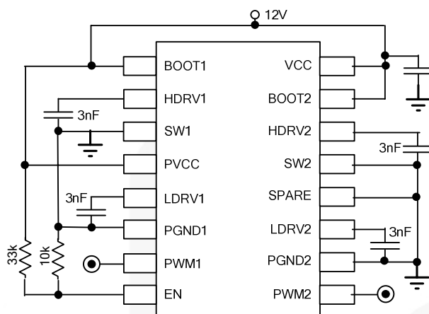
Figure 4. Test Circuit
