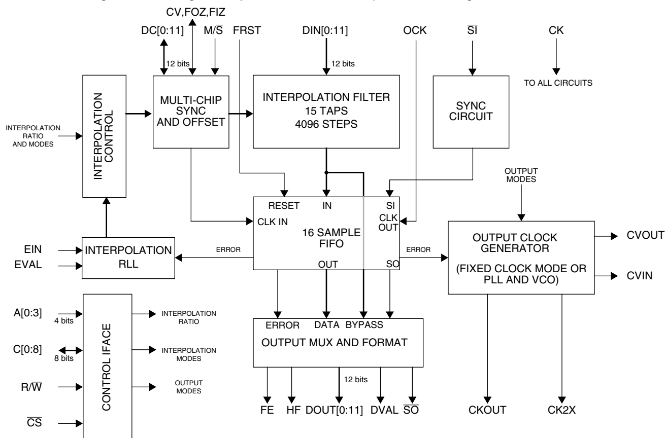
Figure 1. GC3011 Block Diagram
