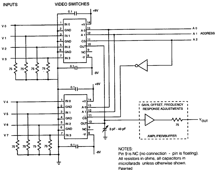
Fig. 6 Video Multiplexer Incorporating Two GX414As
