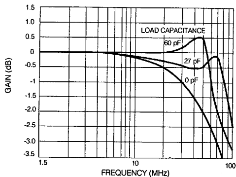
Fig. 3 Gain vs Frequency
