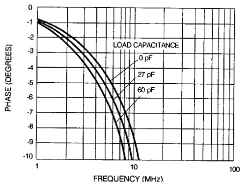
Fig. 2 Phase vs Frequency
