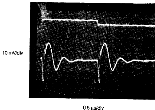
Fig. 4 Switching Transient (crosspoint-to-crosspoint)
