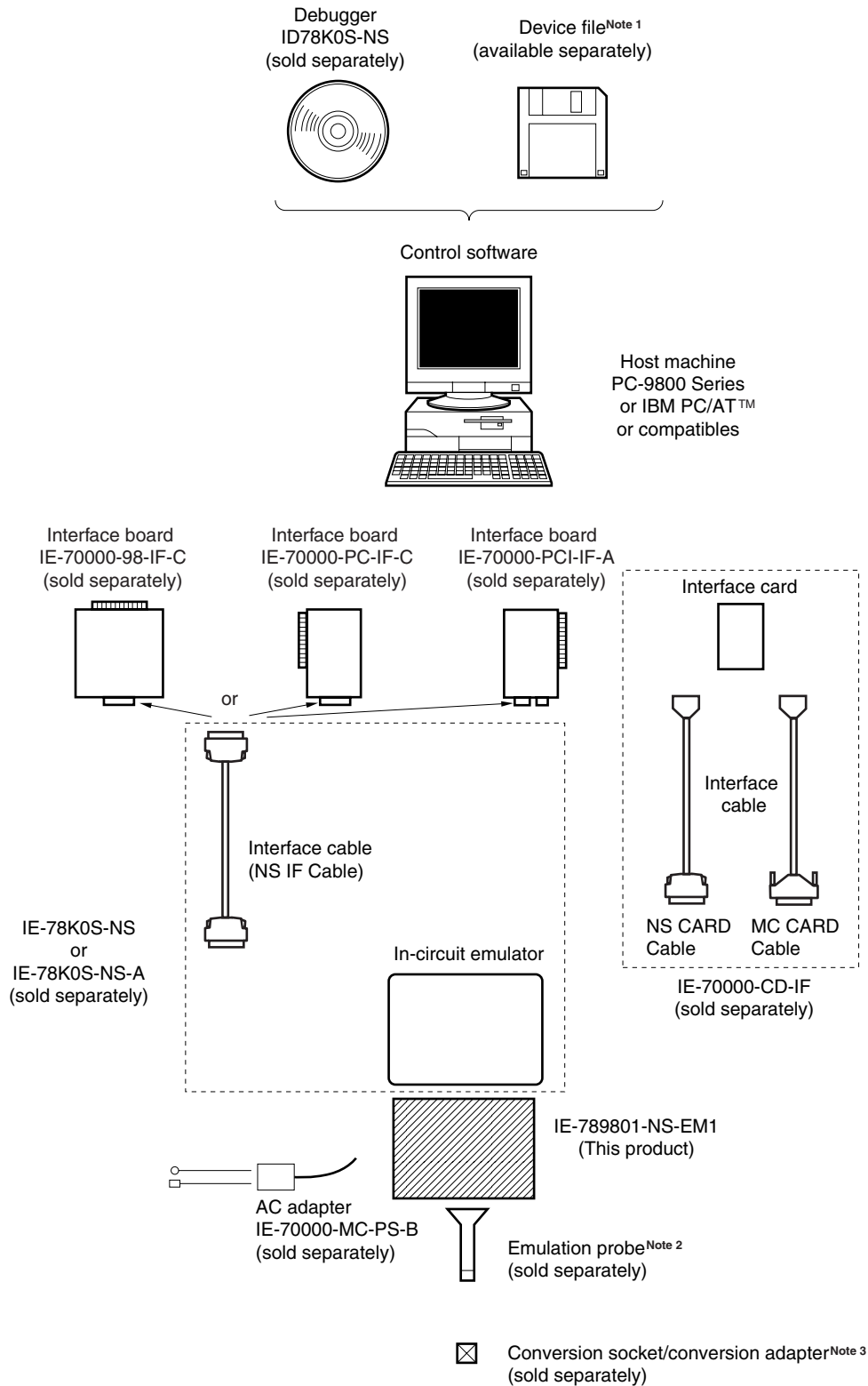
Figure 1-1. System Configuration
