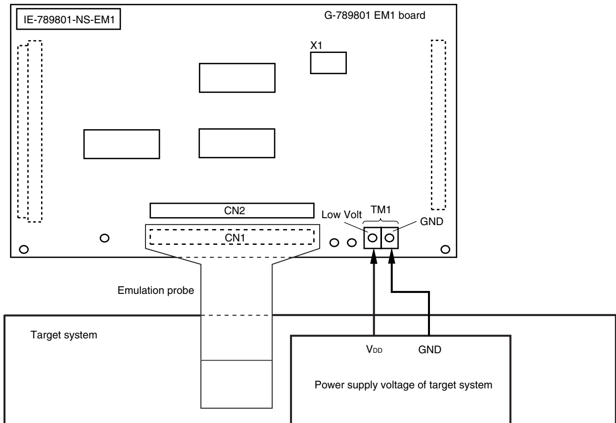
Figure 3-9. Connection of TM1 and Power Supply Voltage of Target System
