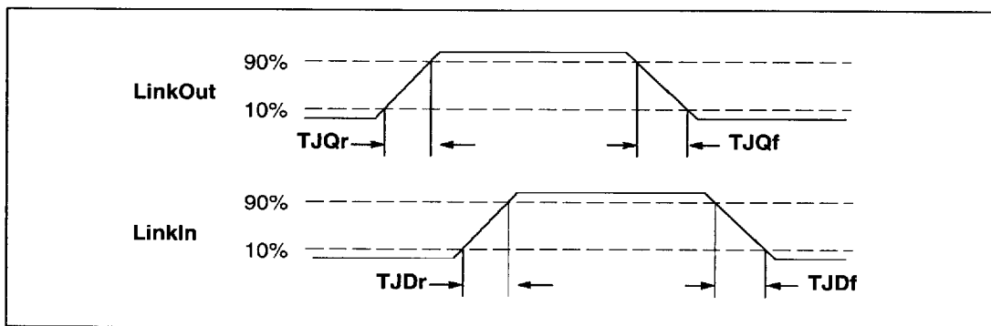
Figure 4.2 IMS C011E link timing
