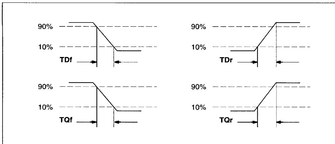
Figure 7.3 IMS C011E input and output edge timing
