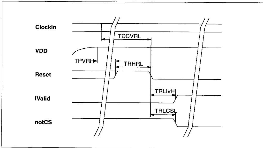
Figure 3.3 Reset timing
