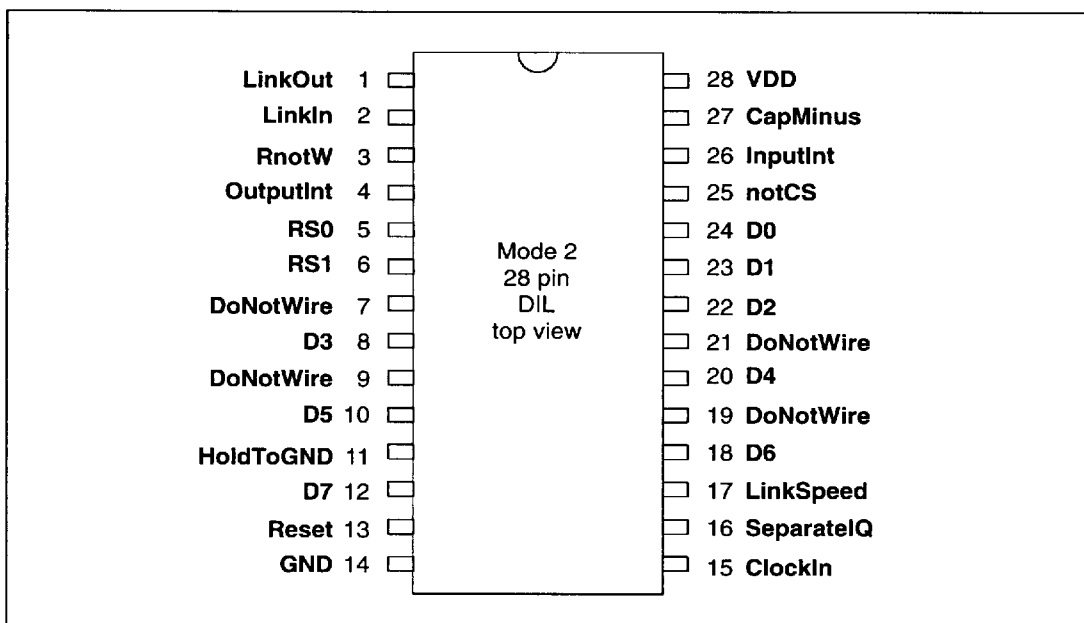
Figure 8.2 IMS C011E Mode 2 28 pin DIL package pinout
