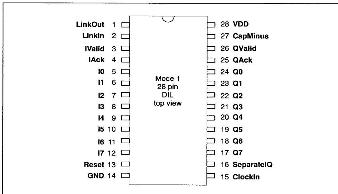
Figure 8.1 IMS C011E Mode 1 28 pin DIL package pinout
