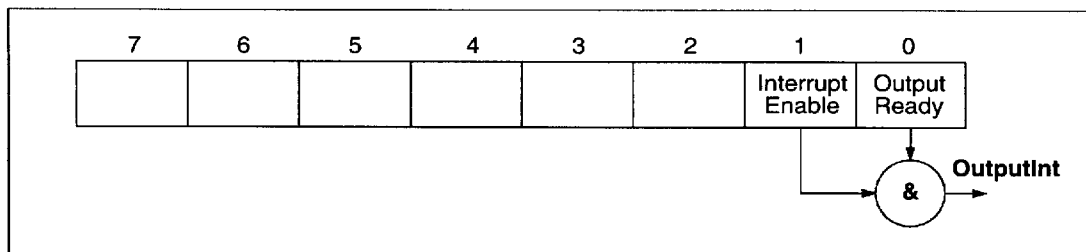
Figure 6.4 IMS C011E Mode 2 output status register
