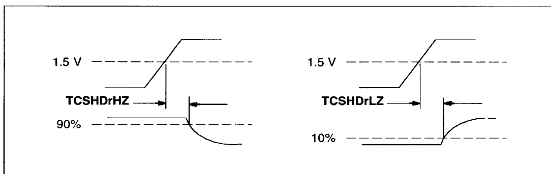
Figure 7.4 IMS C011E tristate timing relative to notCS
