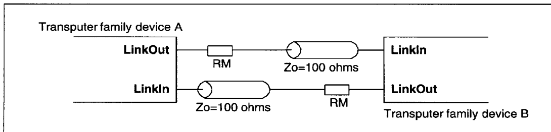
Figure 4.5 Links connected by transmission line
