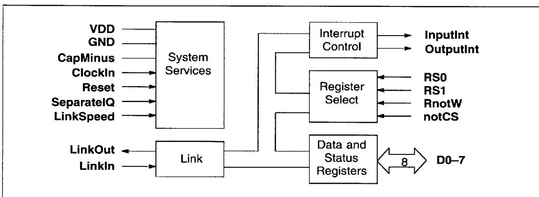
Figure 1.2 IMS C011E Mode 2 block diagram
