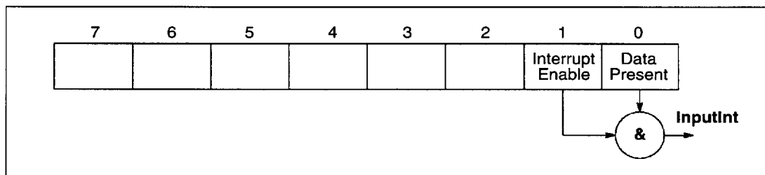
Figure 6.3 IMS C011E Mode 2 input status register
