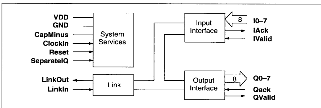
Figure 1.1 IMS C011E Mode 1 block diagram
