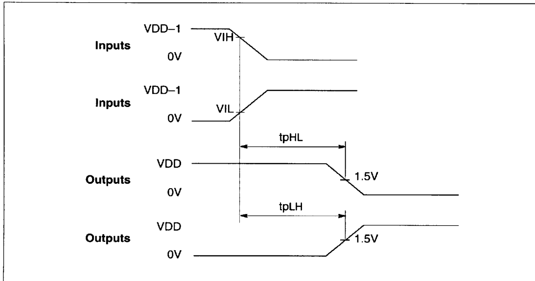
Figure 7.2 AC measurements timing waveforms
