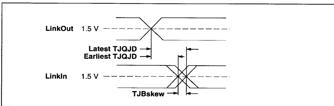
Figure 4.3 IMS C011E buffered link timing
