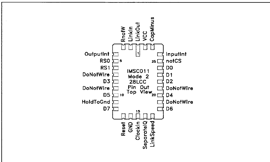
Figure 8.5 IMS C011E Mode 2 28 pin LCC package pinout
