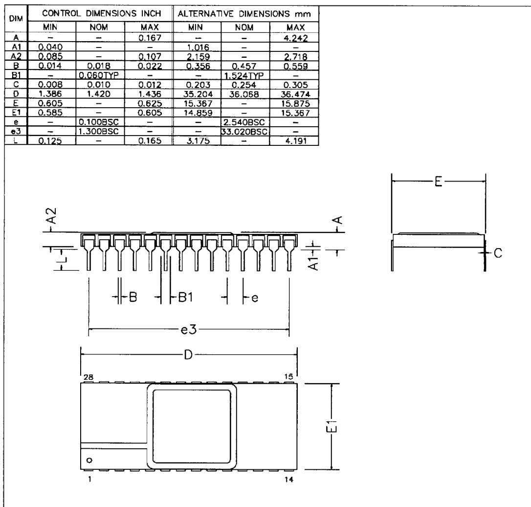
Figure 8.3 28 pin ceramic dual-in-line package dimensions
