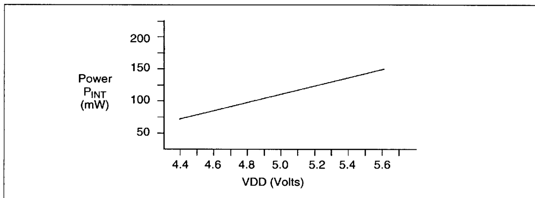
Figure 7.6 IMS C011E internal power dissipation vs VDD
