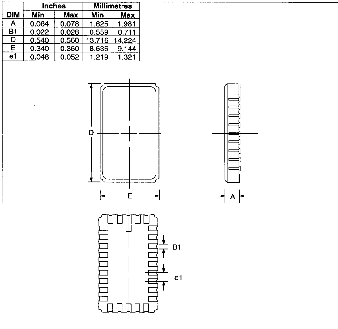
Figure 8.6 28 pin leadless chip carrier package dimensions
