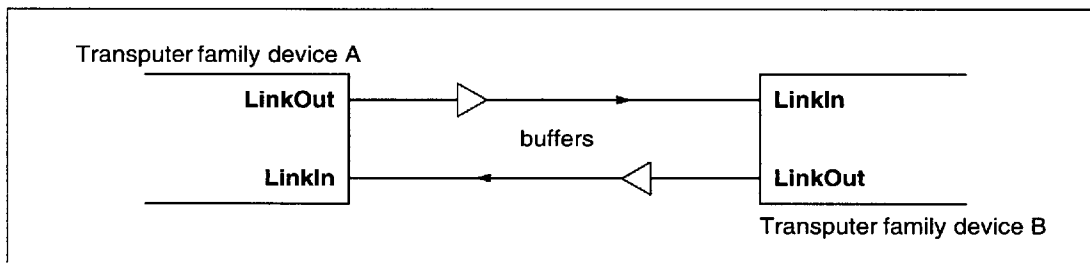
Figure 4.6 Links connected by buffers
