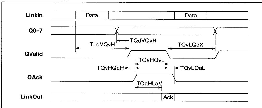
Figure 5.2 IMS C011E Mode 1 parallel data output from link adaptor
