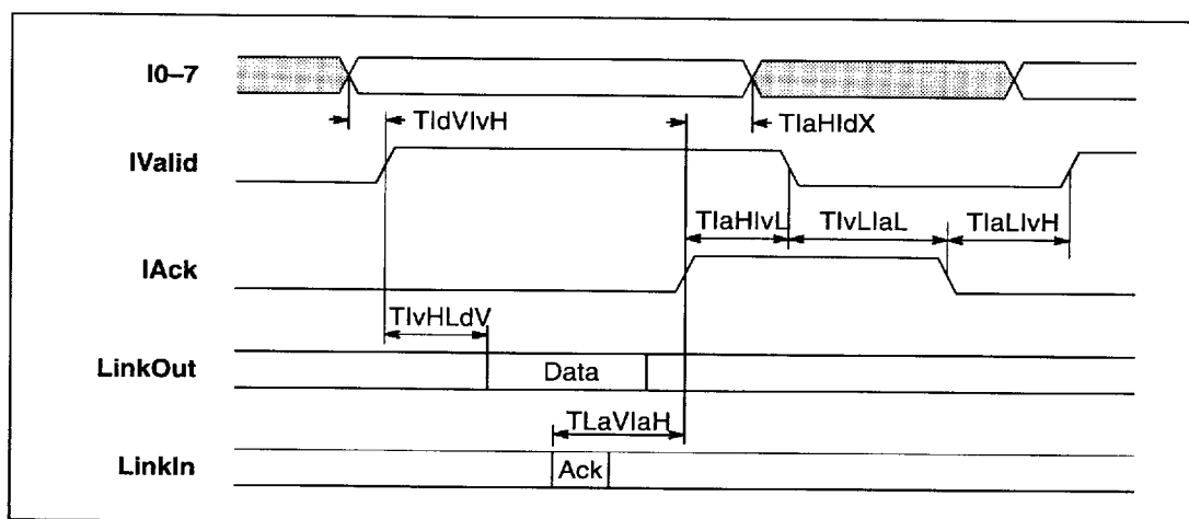
Figure 5.1 IMS C011E Mode 1 parallel data input to link adaptor
