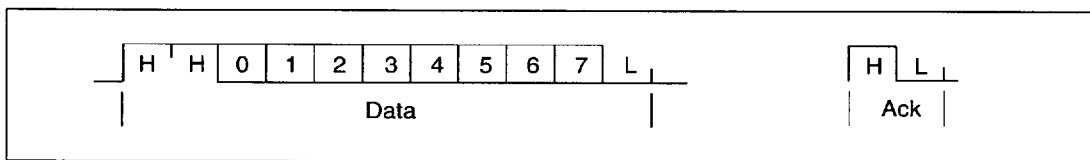
Figure 4.1 IMS C011E link data and acknowledge packets
