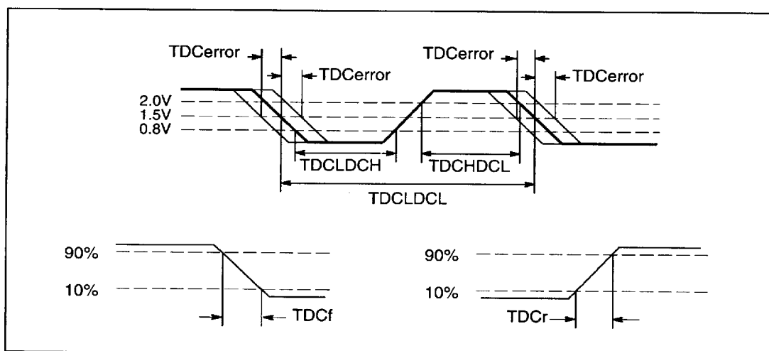
Figure 3.2 ClockIn timing
