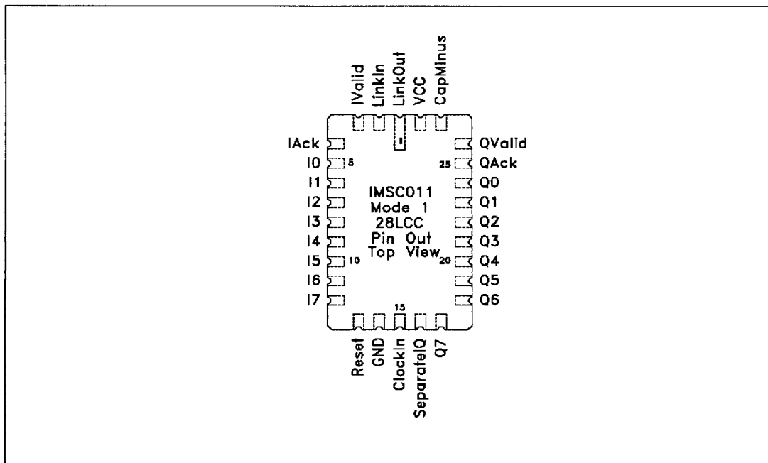
Figure 8.4 IMS C011E Mode 1 28 pin LCC package pinout
