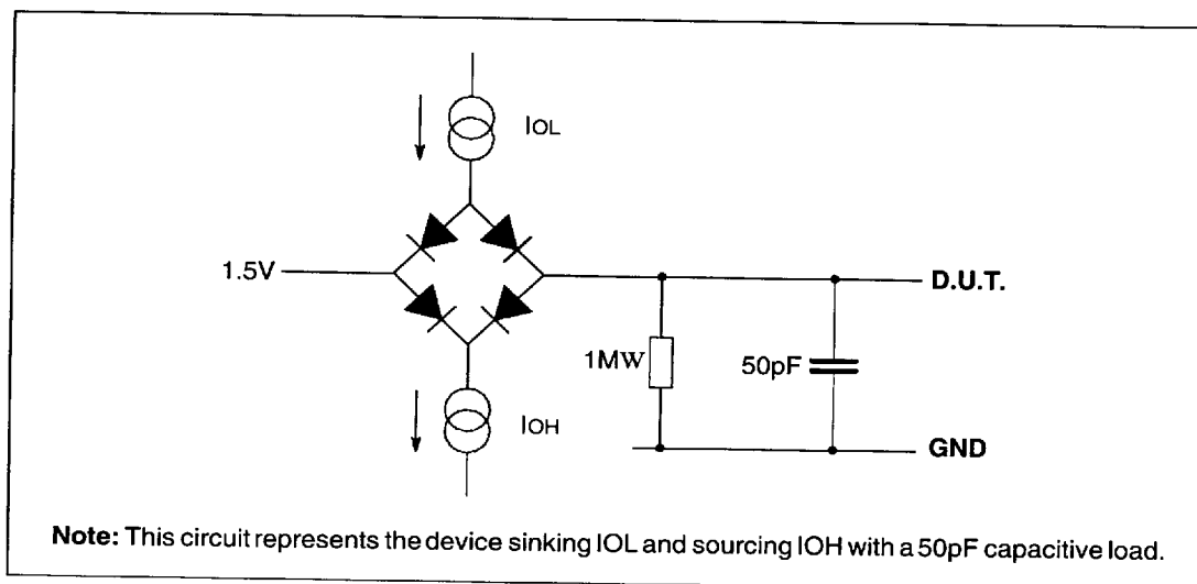
Figure 7.1 Load circuit for AC measurements
