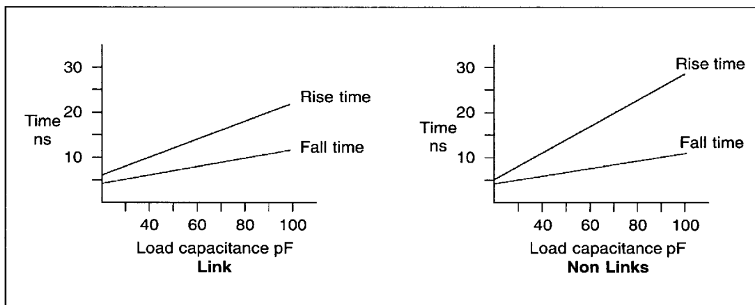
Figure 7.5 Typical rise/fall times
