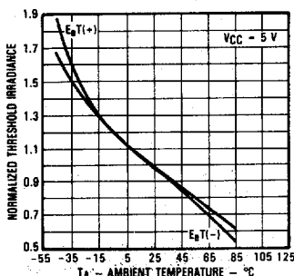
Normalized Threshold Irradiance vs. Amb. Temp.
