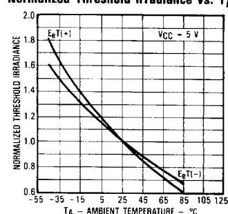
Normalized Threshold Irradiance vs. T_A
