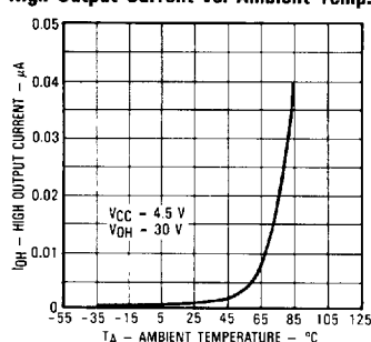
High Output Current vs. Ambient Temp.
