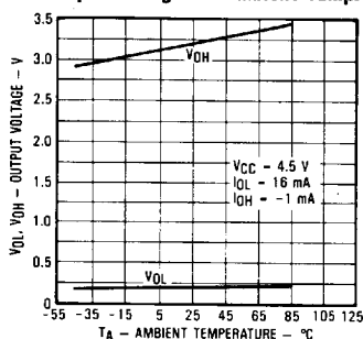
Output Voltage vs. Ambient Temp.
