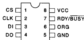
8-Pin PDIP
