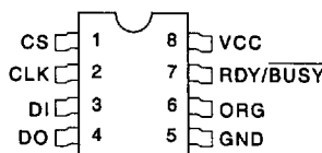
8-Pin SOIC
