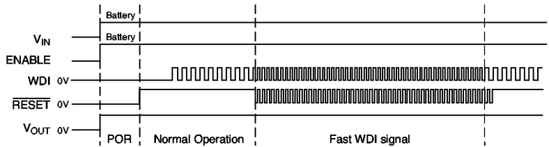
3e: WDI held high after a normal period of operation; ENABLE = LOW.
