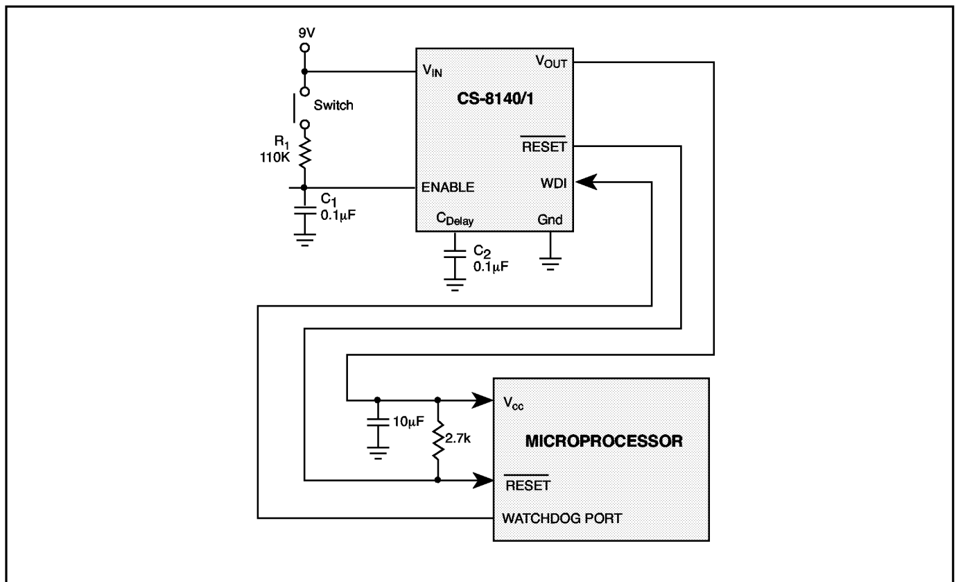
Figure 8. Applications diagram for CS-8140. The CS-8140 provides a 5V tightly regulated supply and control function to the microprocessor. In this application, the microprocessor controls its own power down sequence (see text).
