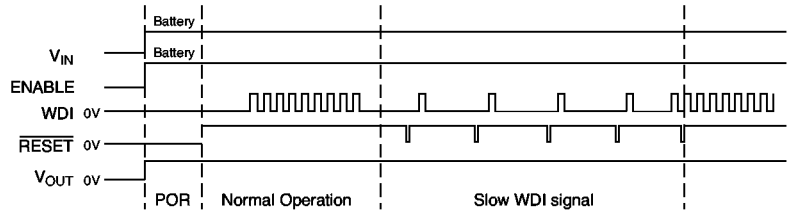
3d: V_{OUT} when Watchdog is too fast and ENABLE = HIGH.
