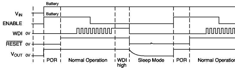
3f: WDI held low or is too slow after a normal period of operation; ENABLE = LOW.
