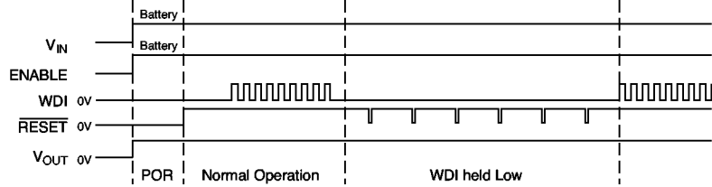
3c: V_{OUT} when Watchdog is too slow and ENABLE = HIGH.
