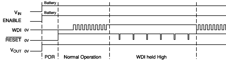
3b: V_{OUT} when Watchdog is held low and ENABLE = HIGH.
