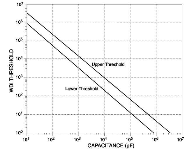
Watchdog Frequency Threshold vs. C_{DELAY}
