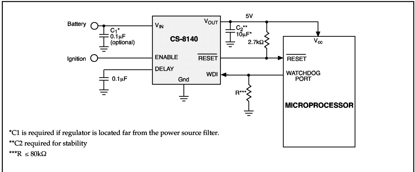
Figure 7. Application Diagram
