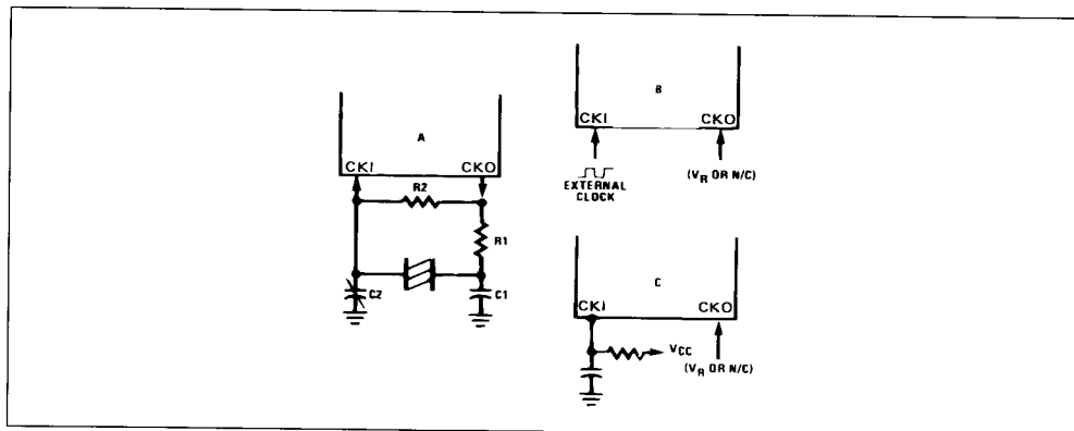
Figure 6 : ETL9410/L9411 Oscillator.
