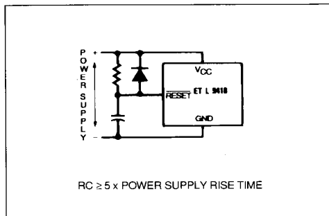
Figure 5 : Power-up Clear Circuit.
