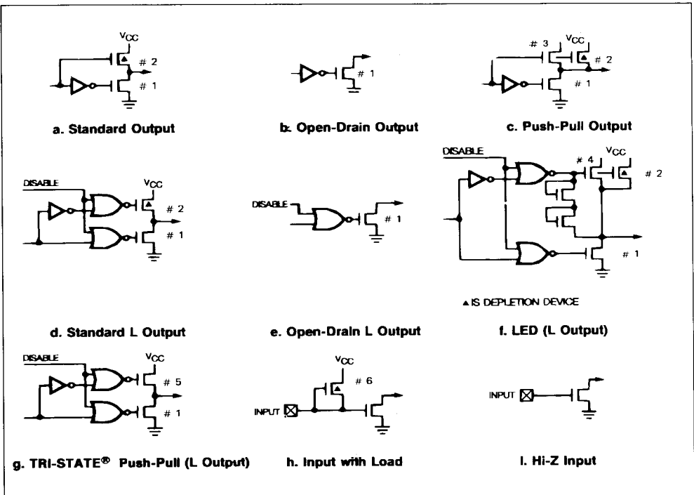
Figure 7 : Input and Output Configurations.
