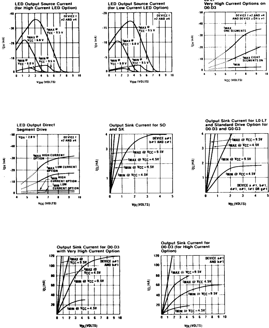
Figure 8a : ETL9410/L9411 - I/O DC Current Characteristics (continued).
