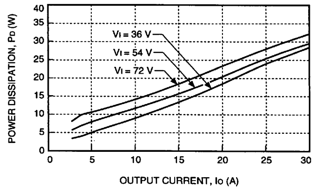
Figure 20. Power Dissipation as Heat vs. Output Current
