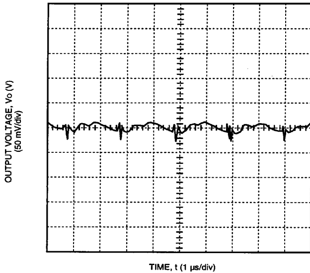
Figure 4. Typical FW150F Output Ripple Voltage at Room Temperature, 48 V Input, and 30 A Output
