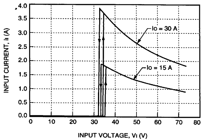
Figure 1. Typical FW150F Input Characteristics at Room Temperature
