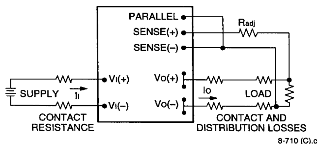
Figure 14. Circuit Configuration to Adjust Output Voltage
