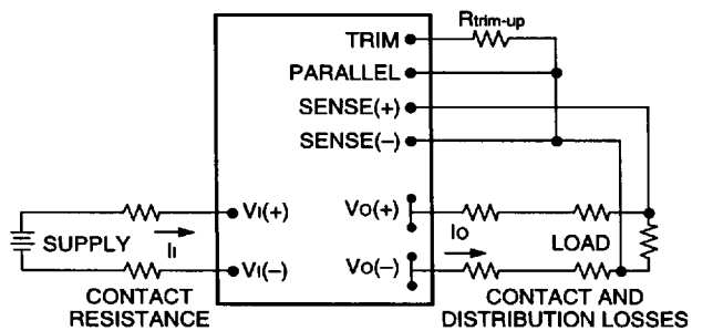
Figure 12. Circuit Configuration to Trim Up Output Voltage
