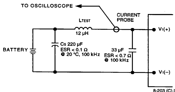
Figure 7. Input Reflected-Ripple Test Setup
