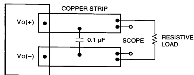
Figure 8. Output Voltage and Efficiency Measurement Test Setup
