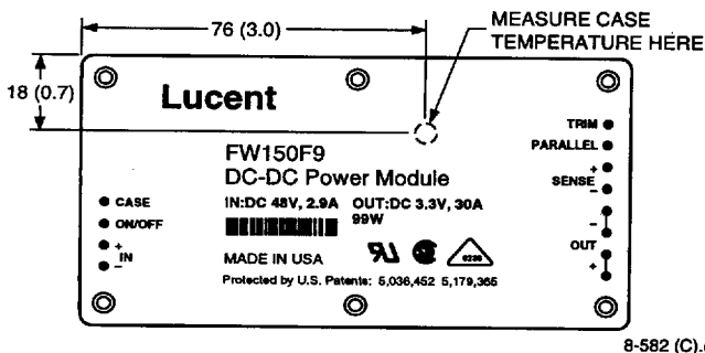
Figure 16. Case Temperature Measurement Location
