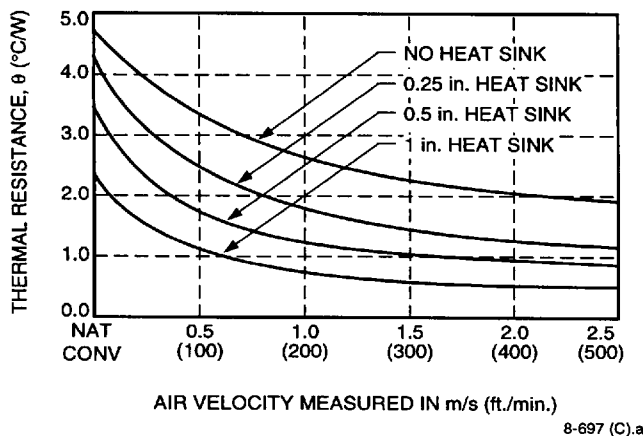
Figure 19. Heat Sink Resistance Curves; Fins Oriented Along Length
