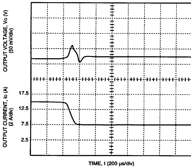
Figure 5. Typical FW150F Transient Response to Step Decrease in Load from 50% to 25% of Full Load at Room Temperature and 48 V Input (Waveform Averaged to Eliminate Ripple Component.)
