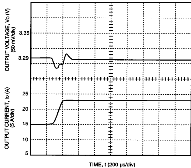
Figure 6. Typical FW150F Transient Response to Step Increase in Load from 50% to 75% of Full Load at Room Temperature and 48 V Input (Waveform Averaged to Eliminate Ripple Component.)
