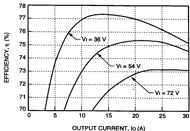
Figure 3. Typical FW150F Efficiency vs. Output Current at Room Temperature
