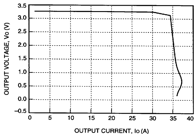
Figure 2. Typical FW150F Output Characteristics at Room Temperature and 48 V Input
