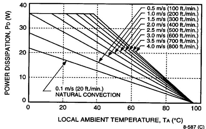
Figure 17. Power Derating vs. Local Ambient Temperature and Air Velocity
