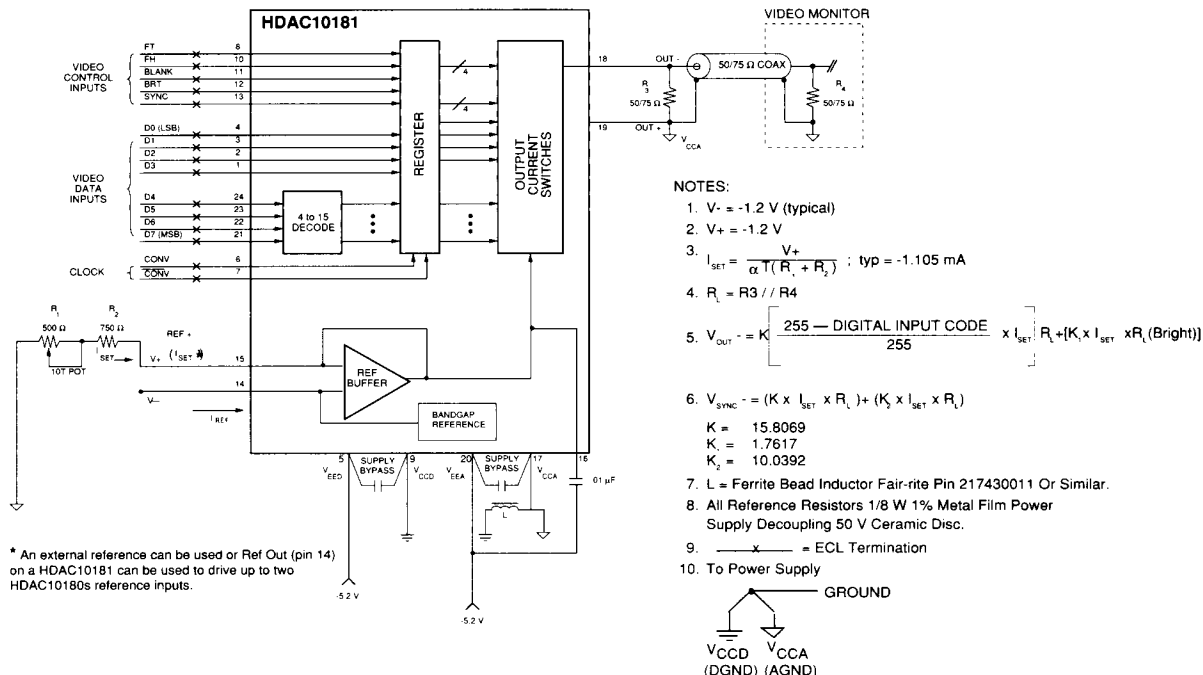
Figure 1 - Typical Interface Circuit
