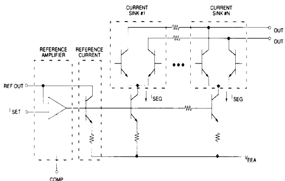
Figure 7 - DAC Output Circuit
