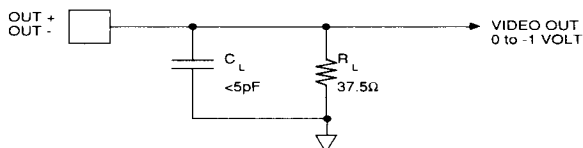
Figure 4B - Test Load
