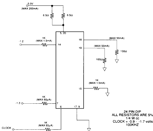
Figure 6 - Burn-In Circuit
