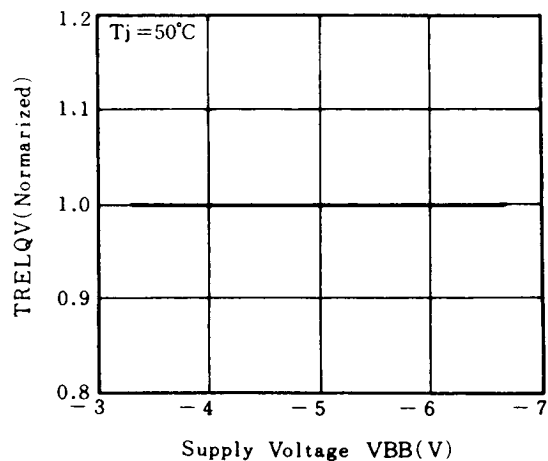
ACCESS TIME (NORMALIZED) vs. VBB
