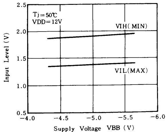
ADDRESS AND DATA INPUT LEVELS vs. VBB
