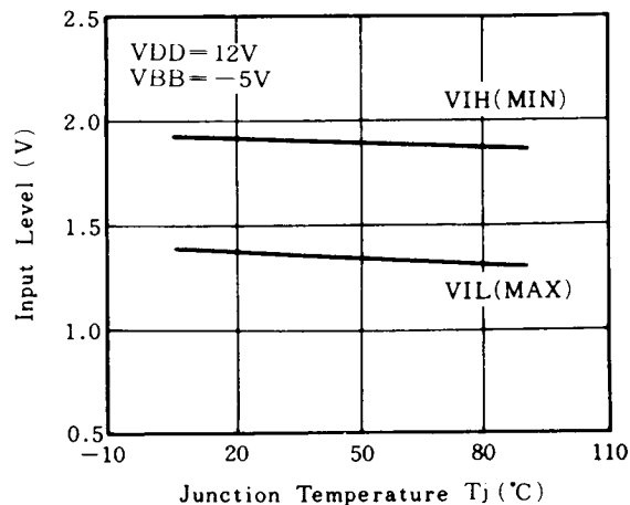
ADDRESS AND DATA INPUT LEVELS vs. Tj
