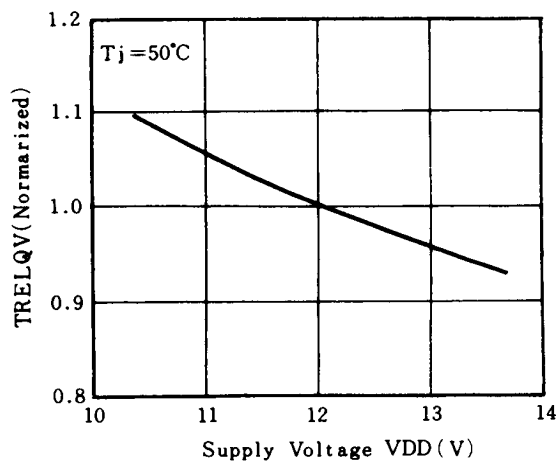
ACCESS TIME (NORMALIZED) vs. VDD
