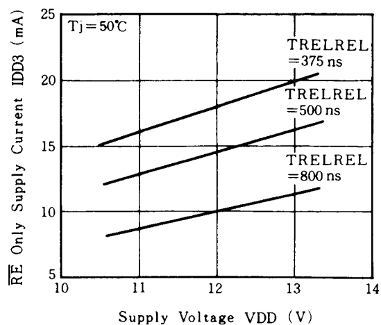
IDD3 ( \overline{RE} ONLY CYCLE) vs. VDD
