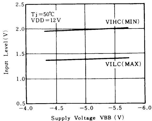
CLOCK INPUT LEVELS vs. VBB
