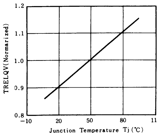
ACCESS TIME (NORMALIZED) vs. Tj
