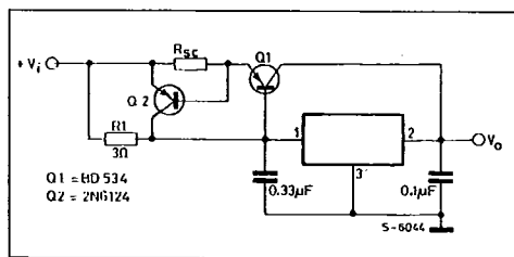
Figure 7 : Short-circuit Protection.
