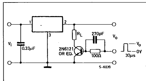
Figure 2 : Load Regulation.
