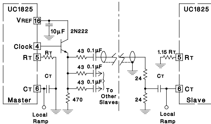
Generalized Synchronization
