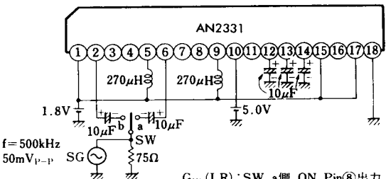
Test Circuit 7 ( G_{V5(LR)} , G_{V5(LB)} )
