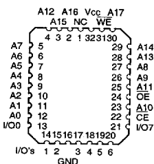
PLCC (1) Top View
