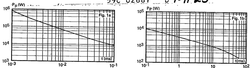
Fig. 1a-1b — Peak pulse power versus exponential pulse duration.
