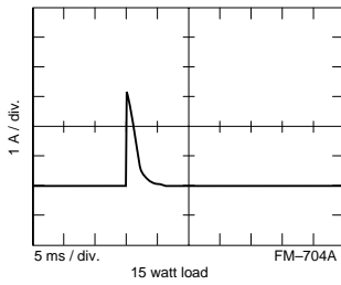
Inrush Current
