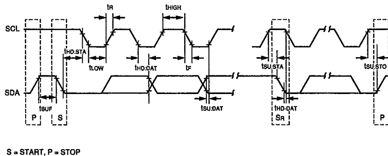
FIGURE 2C - BUS TIMING REQUIREMENTS
