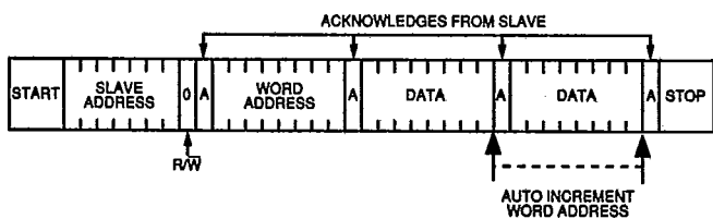
FIGURE 4 - ERASE + REWRITE MODE
