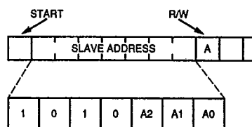
FIGURE 3 - SLAVE ADDRESS ALLOCATION
