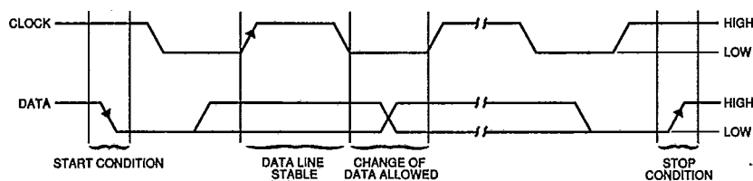
FIGURE 2A - DATA TRANSFER SEQUENCE ON THE SERIAL BUS
