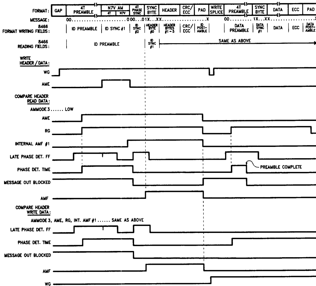
FIGURE 1-4. 4T Preamble, N7V AM (N7V-B Mode)
