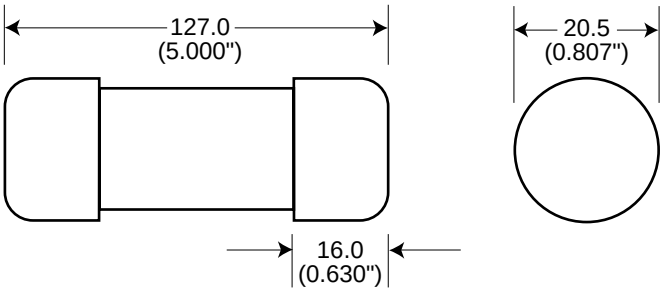
Fig. 2: 35-60 Amp Range
