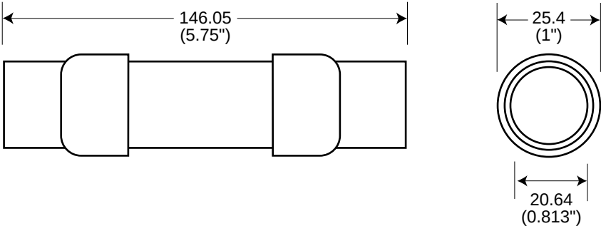
Fig. 2: 35-60 Amp Range
