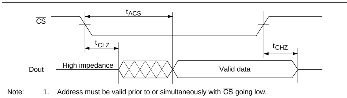
Read Timing Waveform (3) ( \overline{WE} = V_{IH} , \overline{OE} = V_{IL} )*1
