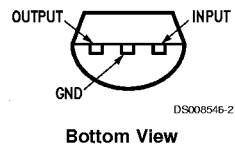
TO-92 Plastic Package (Z)
