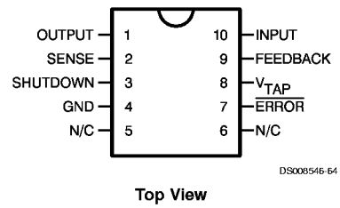
10-Lead Ceramic Surface-Mount Package (WG)
