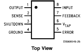
Dual-In-Line Packages (N, J) Surface-Mount Package (M, MM)
