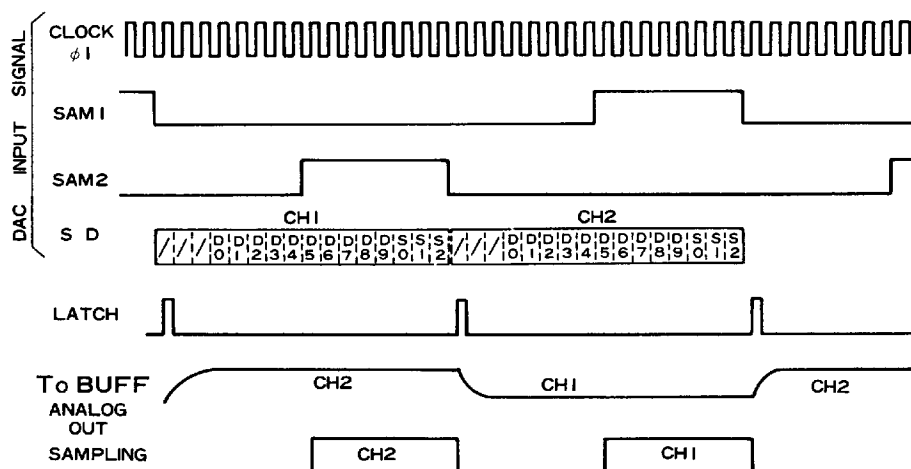
Fig. 3 TIMING
