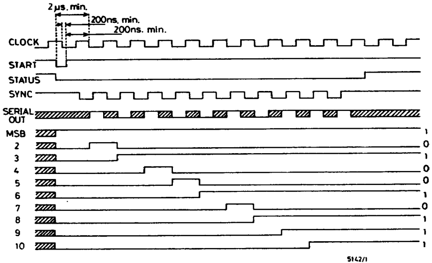
Fig. 5 – TIMING DIAGRAM
