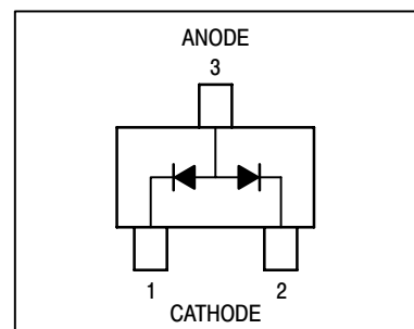
CASE 463-01, STYLE 4 SOT-416/SC-90
