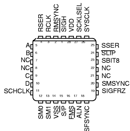
28-PIN PLCC
