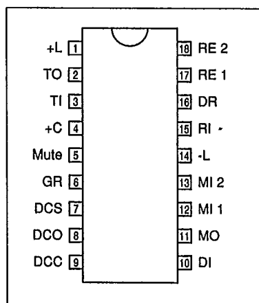
Figure 5. Pin configuration.
