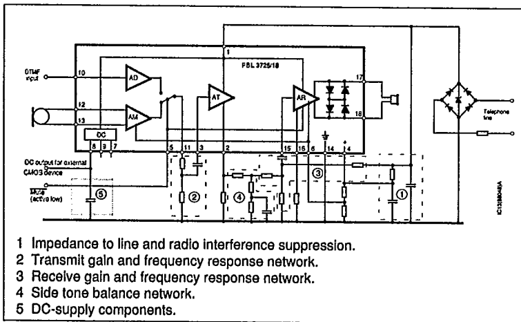
Figure 1. Functional diagram.
