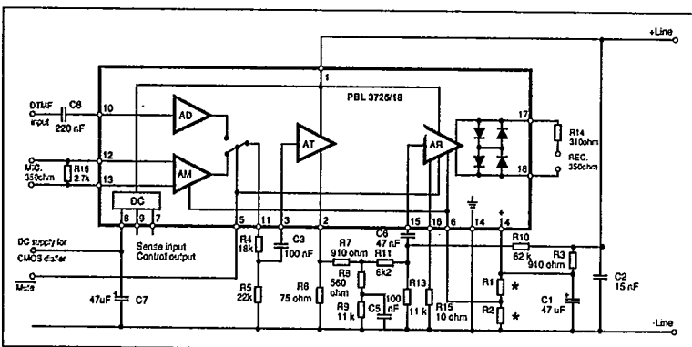
Figure 4. Circuit with external components for test setup.
