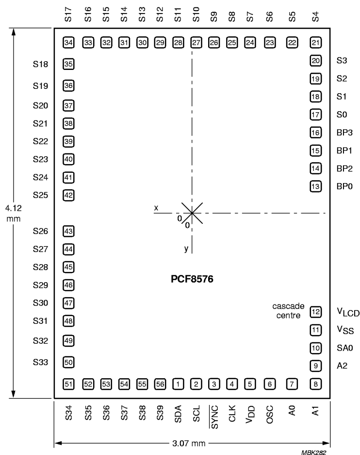
Fig.30 Bonding pad locations.
