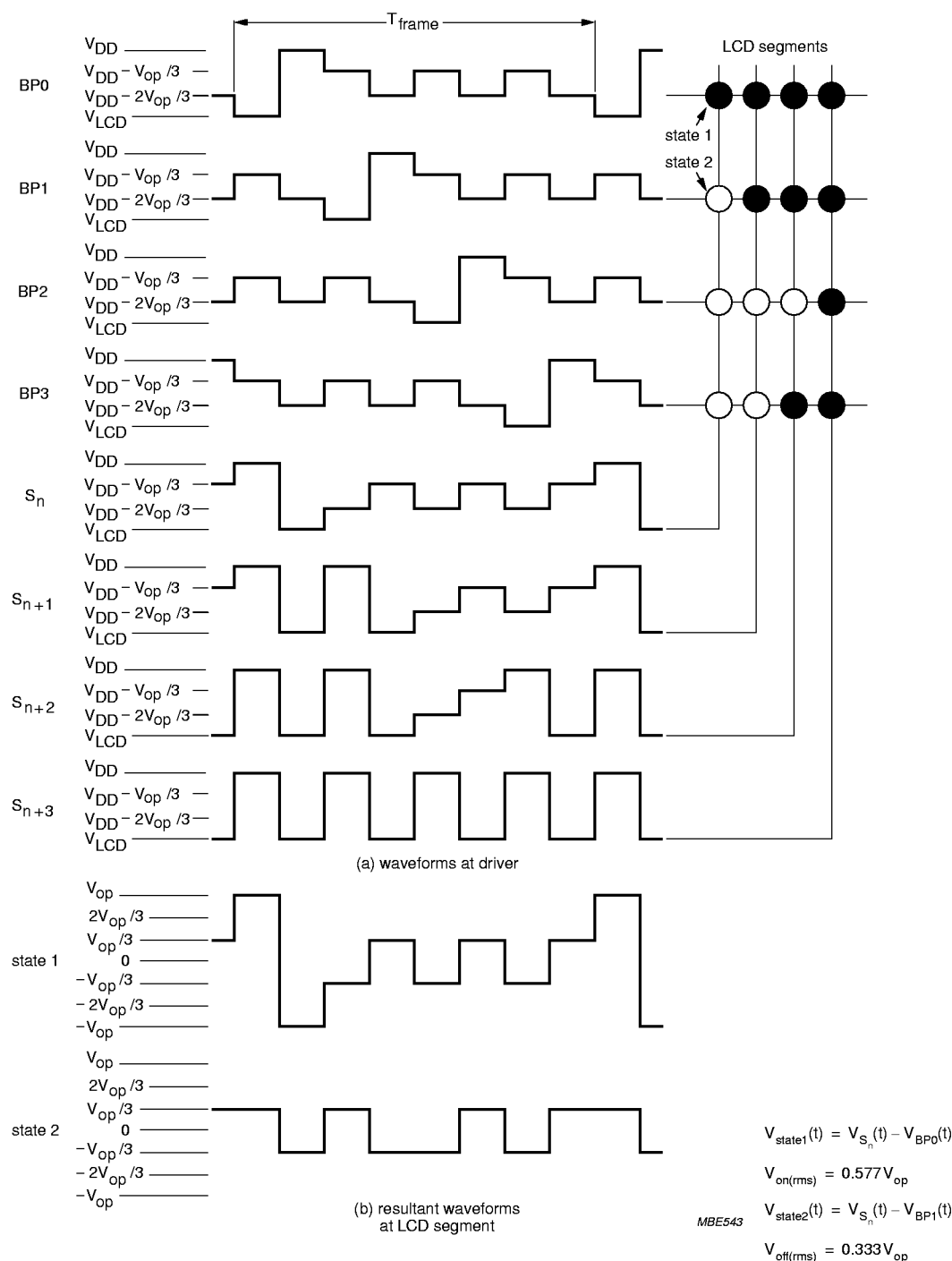
Fig.8 Waveforms for the 1 : 4 multiplex drive mode ( V_{op} = V_{DD} - V_{LCD} ).
