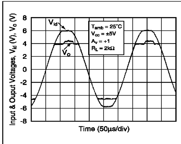
Figure 5 : Behaviour with TSH24
