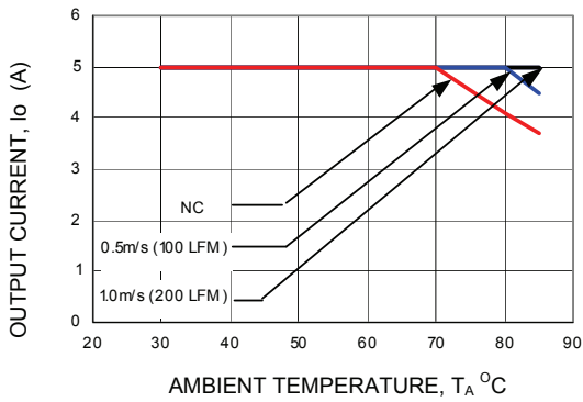
Figure 19. Derating Output Current versus Local Ambient Temperature and Airflow ( V_{in} = 5.0Vdc , V_o=3.3Vdc ).
