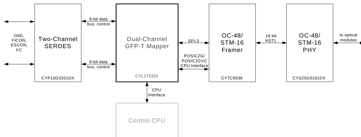
Figure 1. MetroLink2T-2 Application
