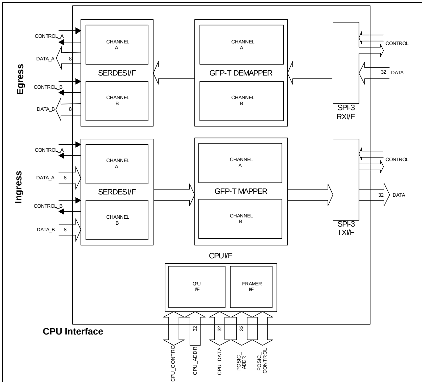
Figure 2. MetroLink2T-2 Top-Level Block Diagram
