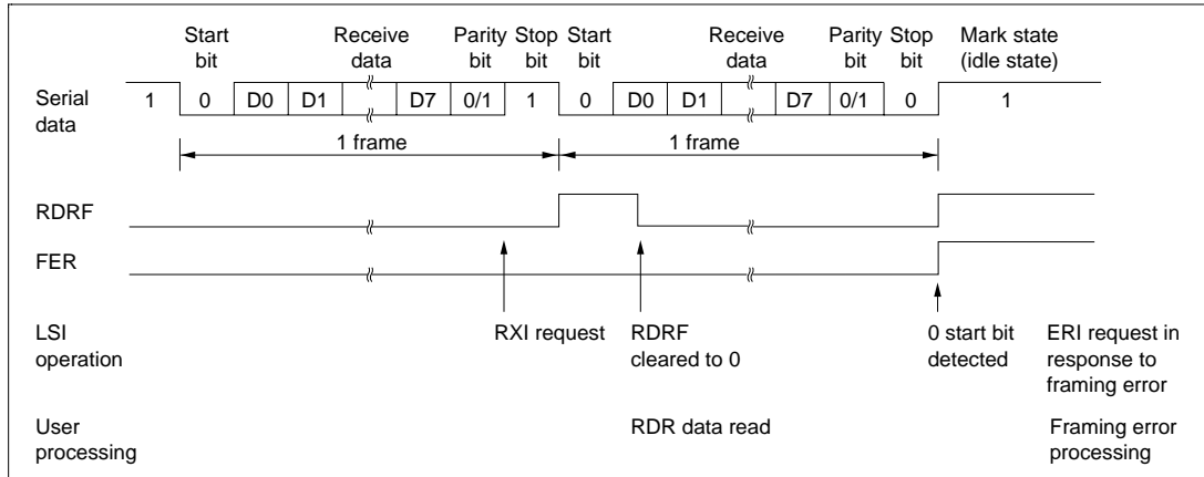
Figure 10.14 Example of Operation when Receiving in Asynchronous Mode (8-Bit Data, Parity, 1 Stop Bit)
