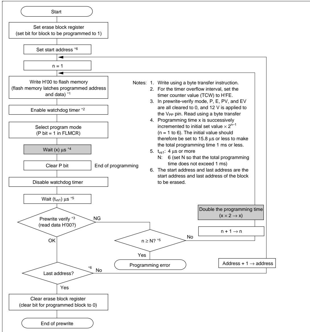
Figure 6.16 Prewrite Flowchart
