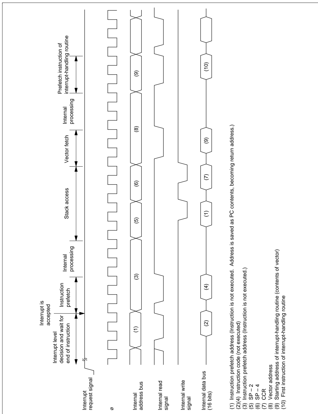
Figure 3.5 Interrupt Sequence
