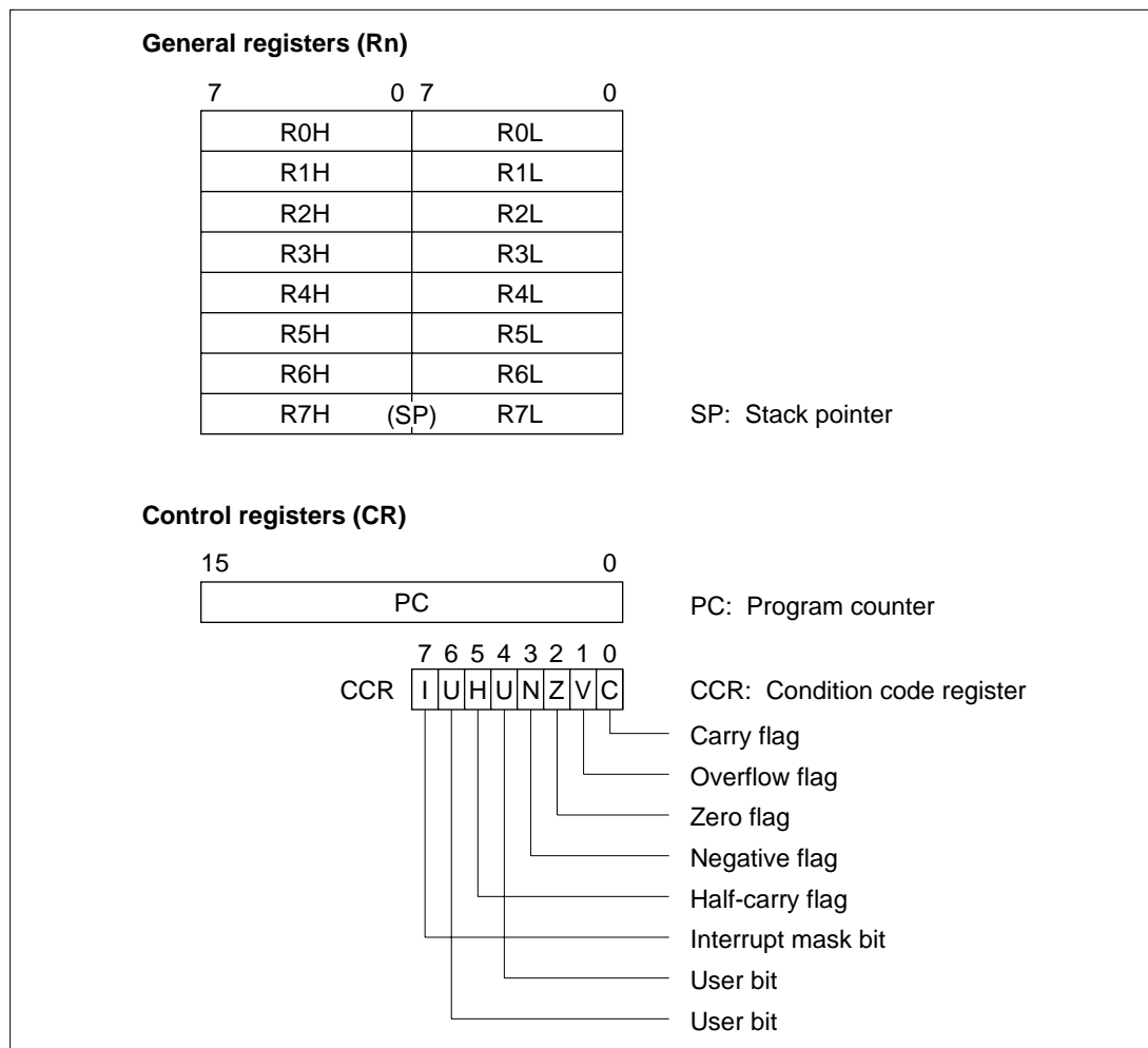
Figure 2.1 CPU Registers
