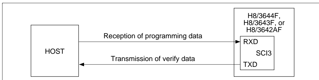
Figure 6.9 Boot Mode System Configuration
