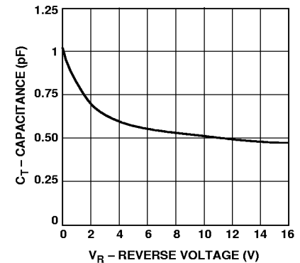
Figure 15. Total Capacitance vs. Reverse Voltage—HSMS-2810 Series.
