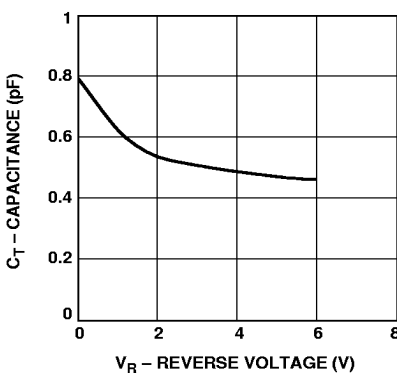
Figure 16. Total Capacitance vs. Reverse Voltage—HSMS-2820 Series.
