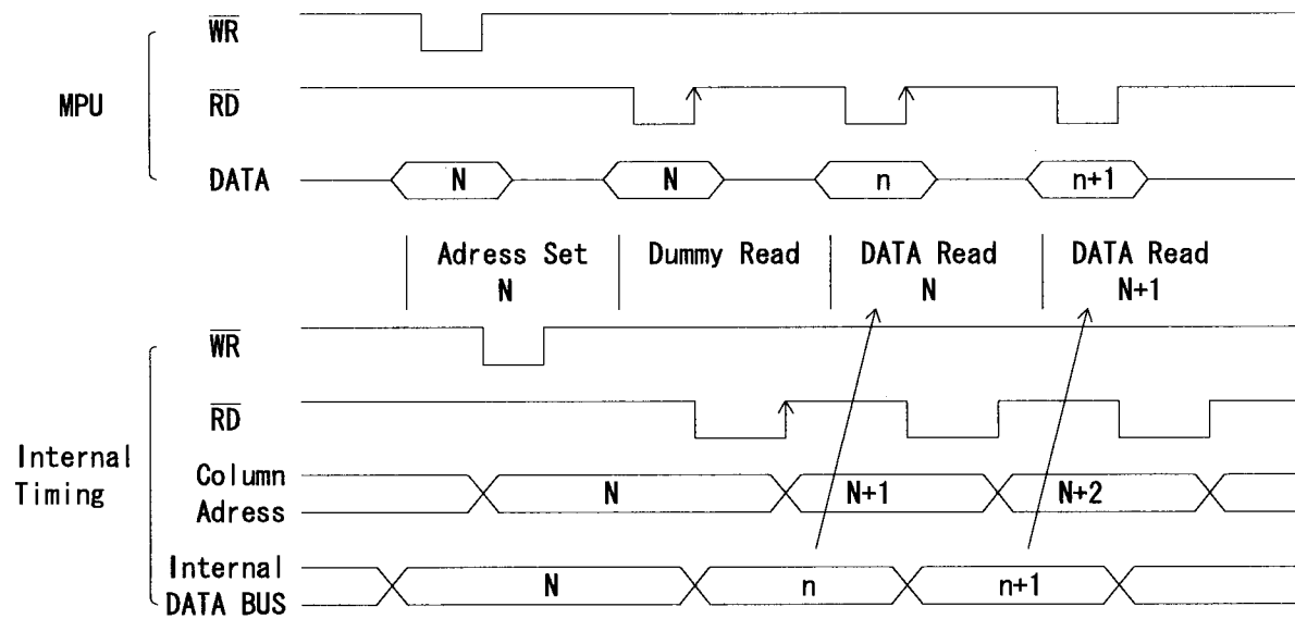
Fig.2 MPU Interface Timing
