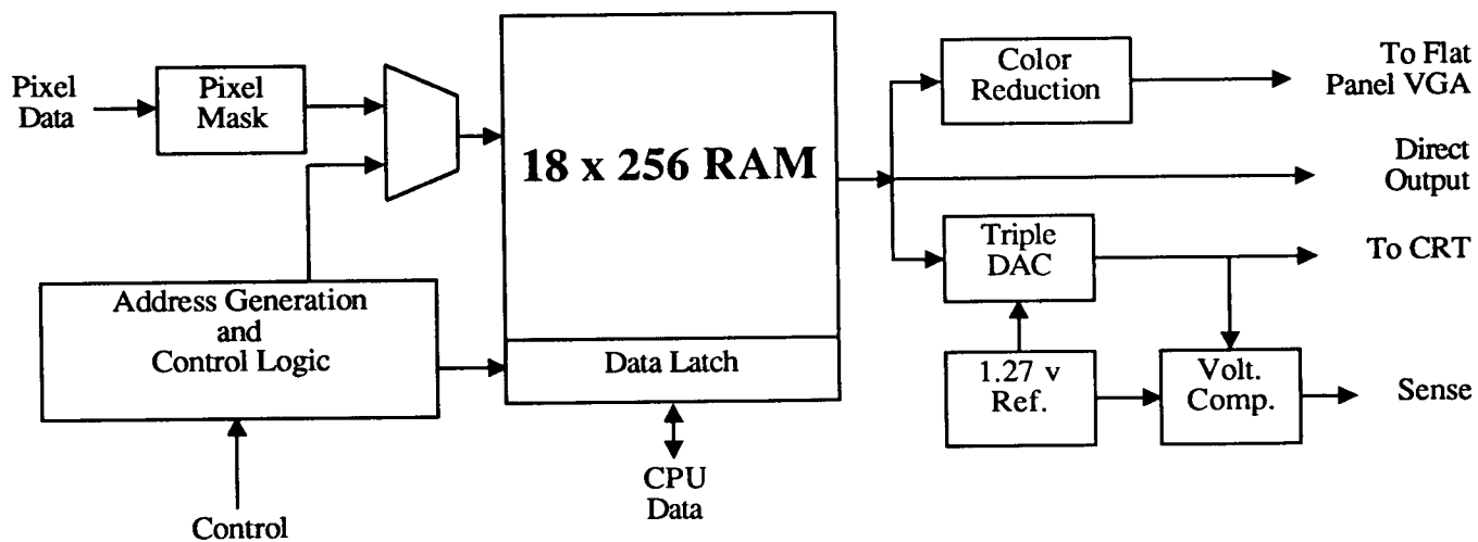
Figure 2-9. 82C411 Block Diagram
