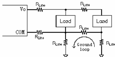
Ground Loops
