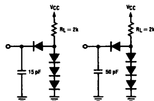
Load Circuit 1
