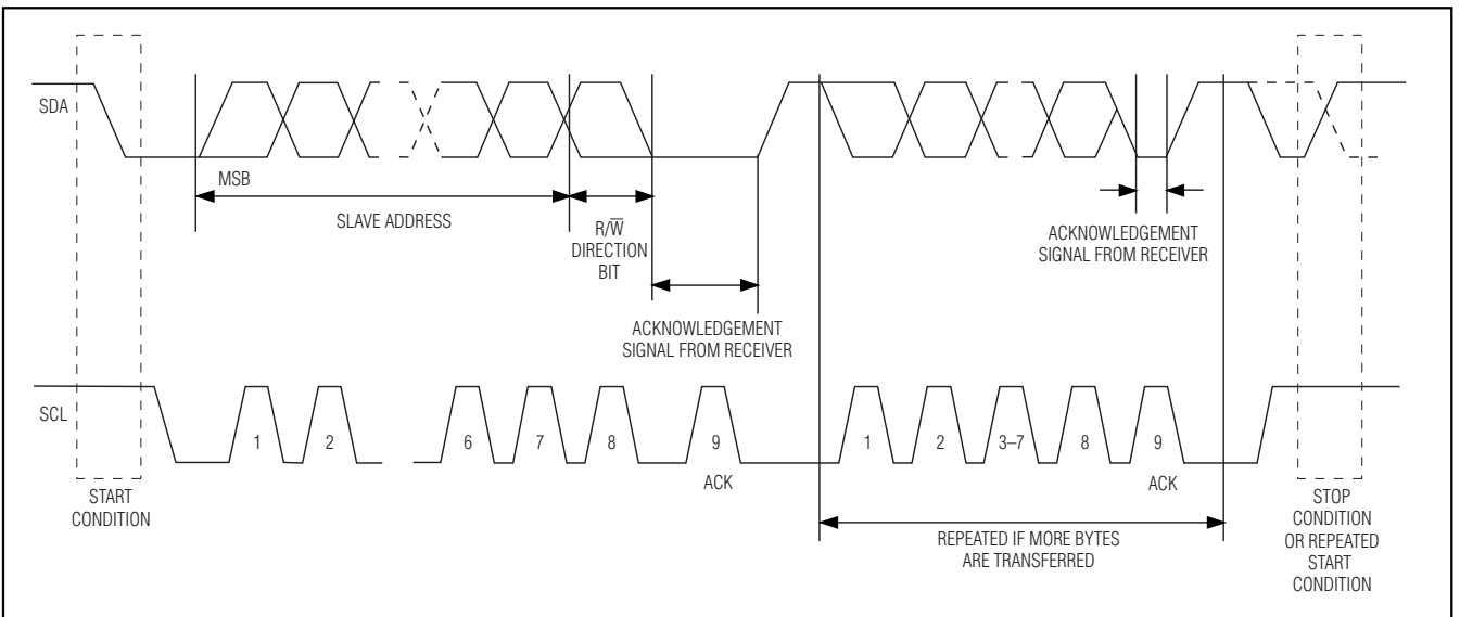
Figure 5. 2-Wire Data Transfer Protocol
