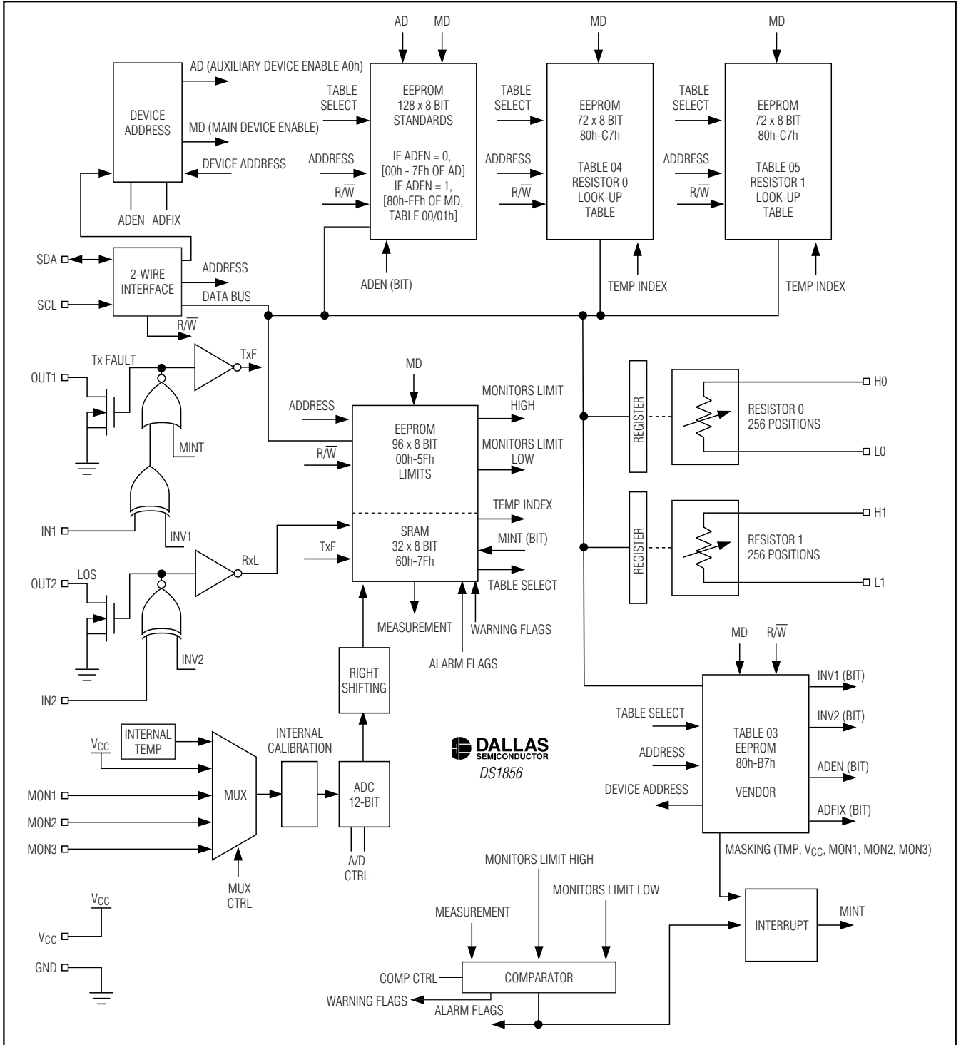
Figure 1. Block Diagram
