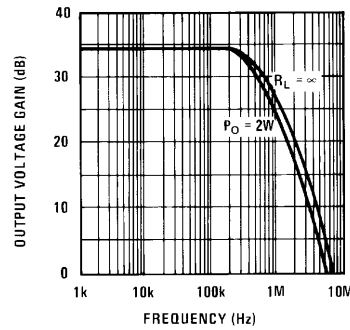
Output Voltage Gain vs Frequency
