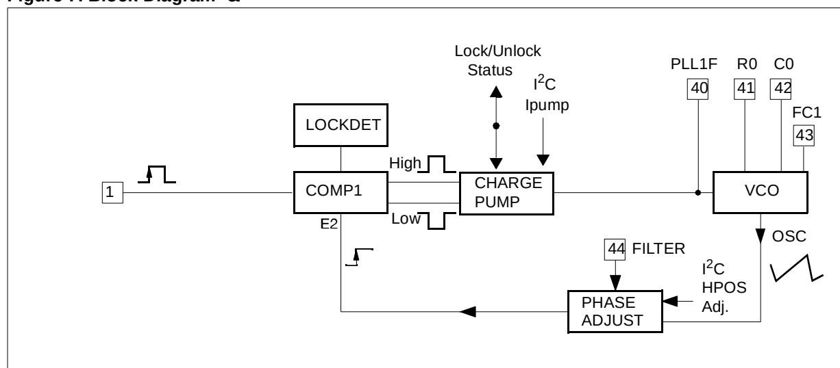
Figure 7. Block Diagram ²&
