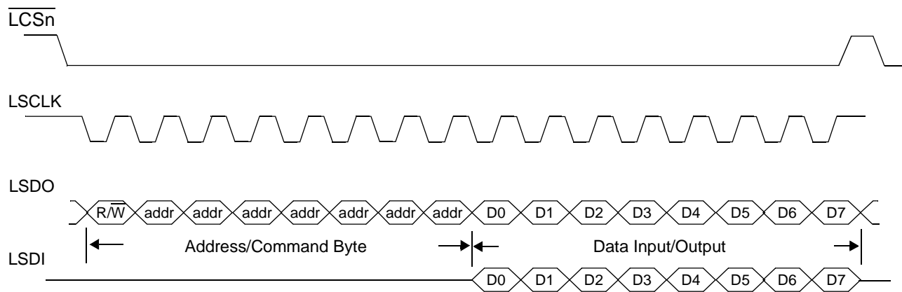
Figure 37. Serial Interface Operation
