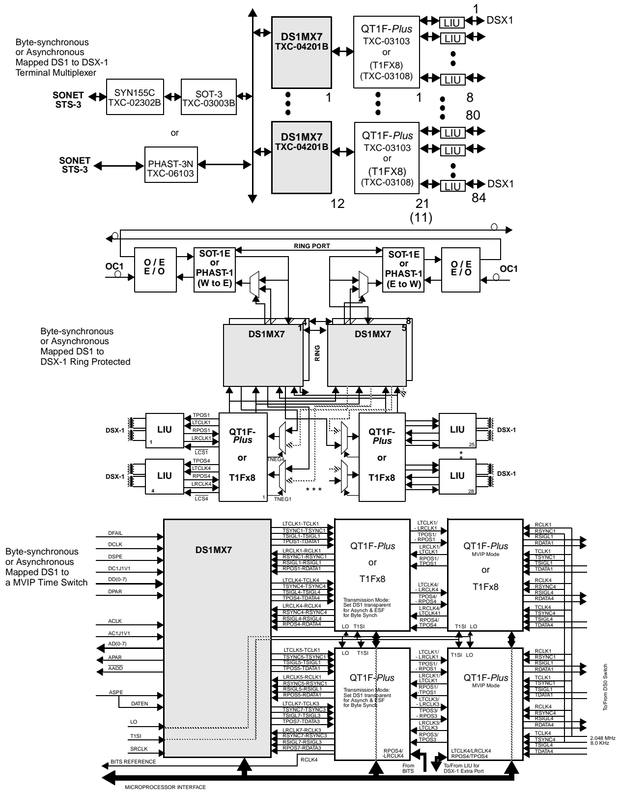
Figure 49. Some DS1MX7 TXC-04201B Byte-synchronous Applications
