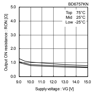
Fig.6 Output ON-Resistance (Linear Constant-Current Drive block)
