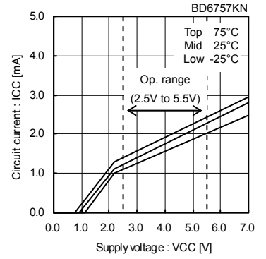
Fig.3 Circuit current
