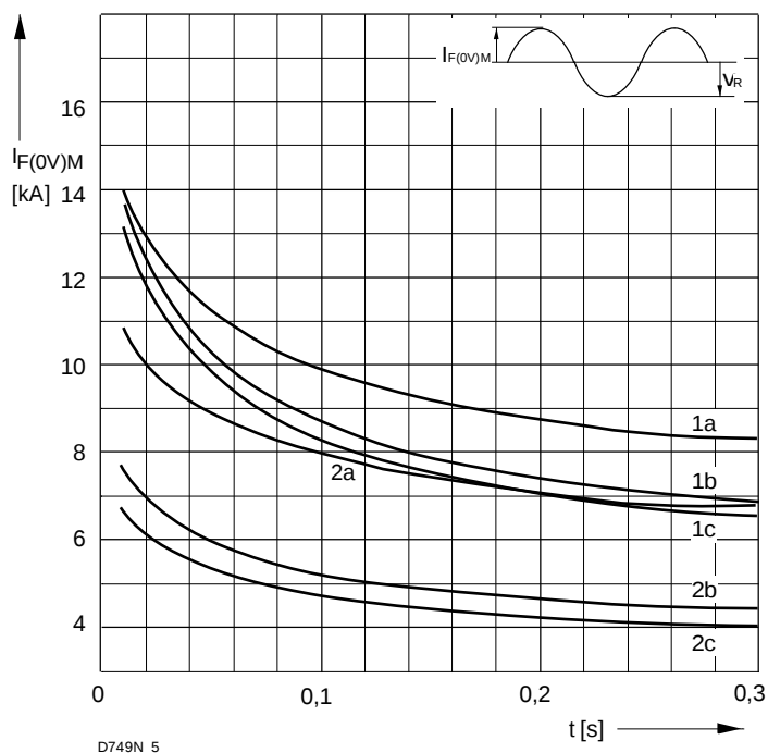
Bild / Fig. 3 Grenzstrom / Maximum overload forward current I_{F(0V)M} = f(t) 1 - I_{FAV(vor)} = 0\text{ A} ; t_j = t_c = 25\text{ °C} 2 - I_{FAV(vor)} = 750\text{ A} ; t_c = 100\text{ °C} ; t_j = 160\text{ °C} a - v_R \leq 50\text{ V} b - v_R = 0,5\text{ }V_{RRM} c - v_R = 0,8\text{ }V_{RRM}
