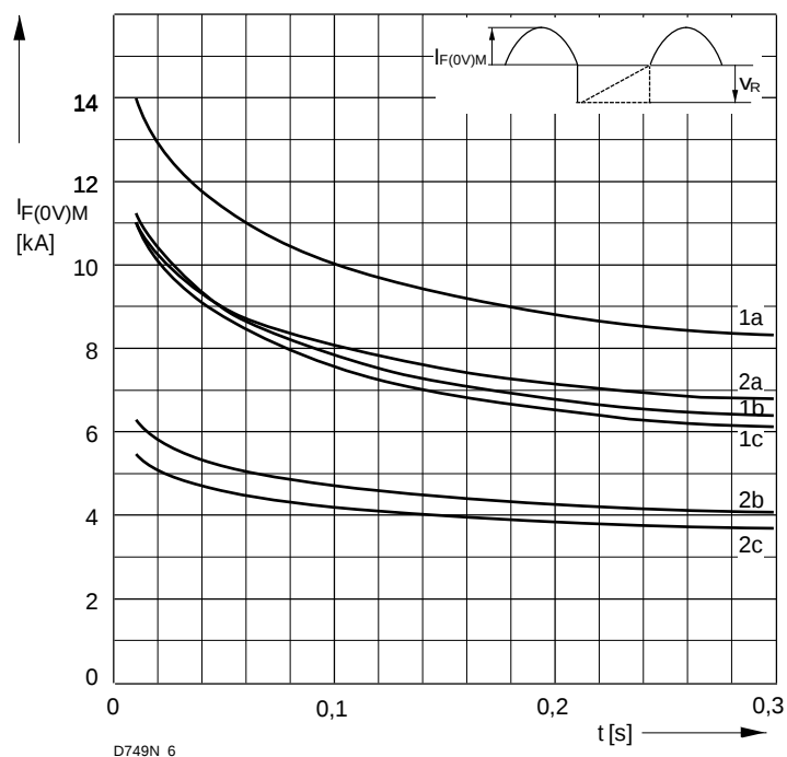
Bild / Fig. 4 Grenzstrom / Maximum overload forward current I_{F(0V)M} = f(t) 1 - I_{FAV(vor)} = 0\text{ A} ; t_j = t_c = 25\text{ °C} 2 - I_{FAV(vor)} = 750\text{ A} ; t_c = 100\text{ °C} ; t_j = 160\text{ °C} a - v_R \leq 50\text{ V} b - v_R = 0,5\text{ }V_{RRM} c - v_R = 0,8\text{ }V_{RRM}
