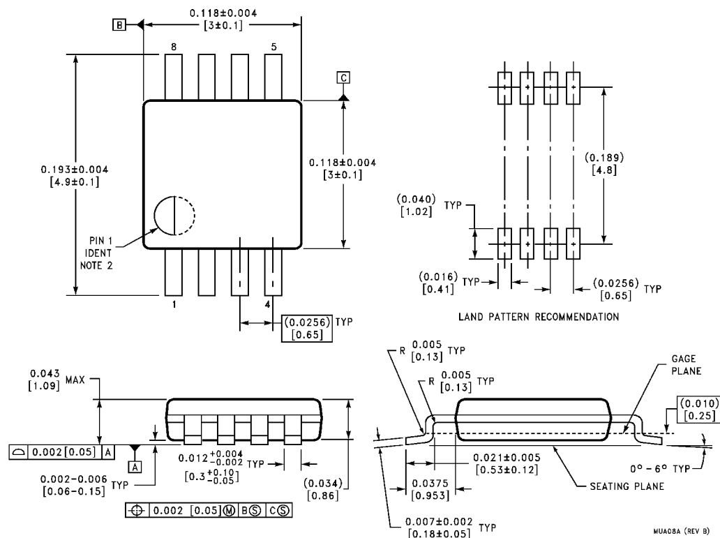
8-Lead Molded Mini Small Outline Package (MSOP) (JEDEC REGISTRATION NUMBER M0-187) Order Number LM66BIMM, LM66BIMMX, LM66CIMM, or LM66CIMMX NS Package Number MUA08A
