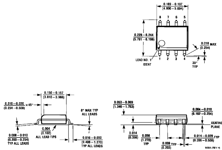
8-Lead (0.150" Wide) Molded Small Outline Package, JEDEC Order Number LM66BIM, LM66BIMX, LM66CIM or LM66CIMX NS Package Number M08A
