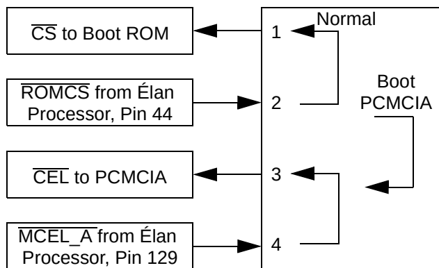
Figure 1. Jumper Configurations
