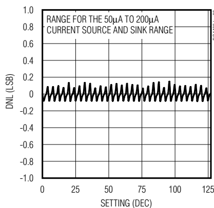
DIFFERENTIAL LINEARITY
