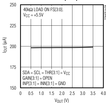
VOLTCO (SINK)
