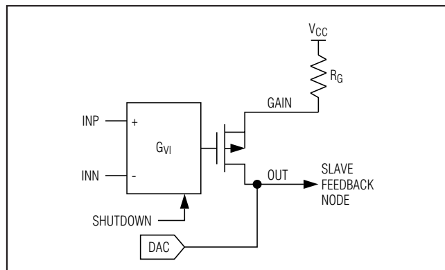
Figure 2. Gain Stage
