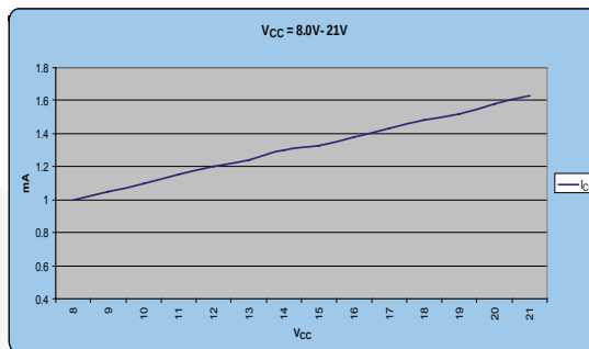
Figure 4. I_{CC} vs. V_{CC} (8.0V-21V) No Load
