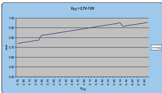
Figure 3. I_{CC} vs. V_{CC} (2.7V-7.0V) No Load
